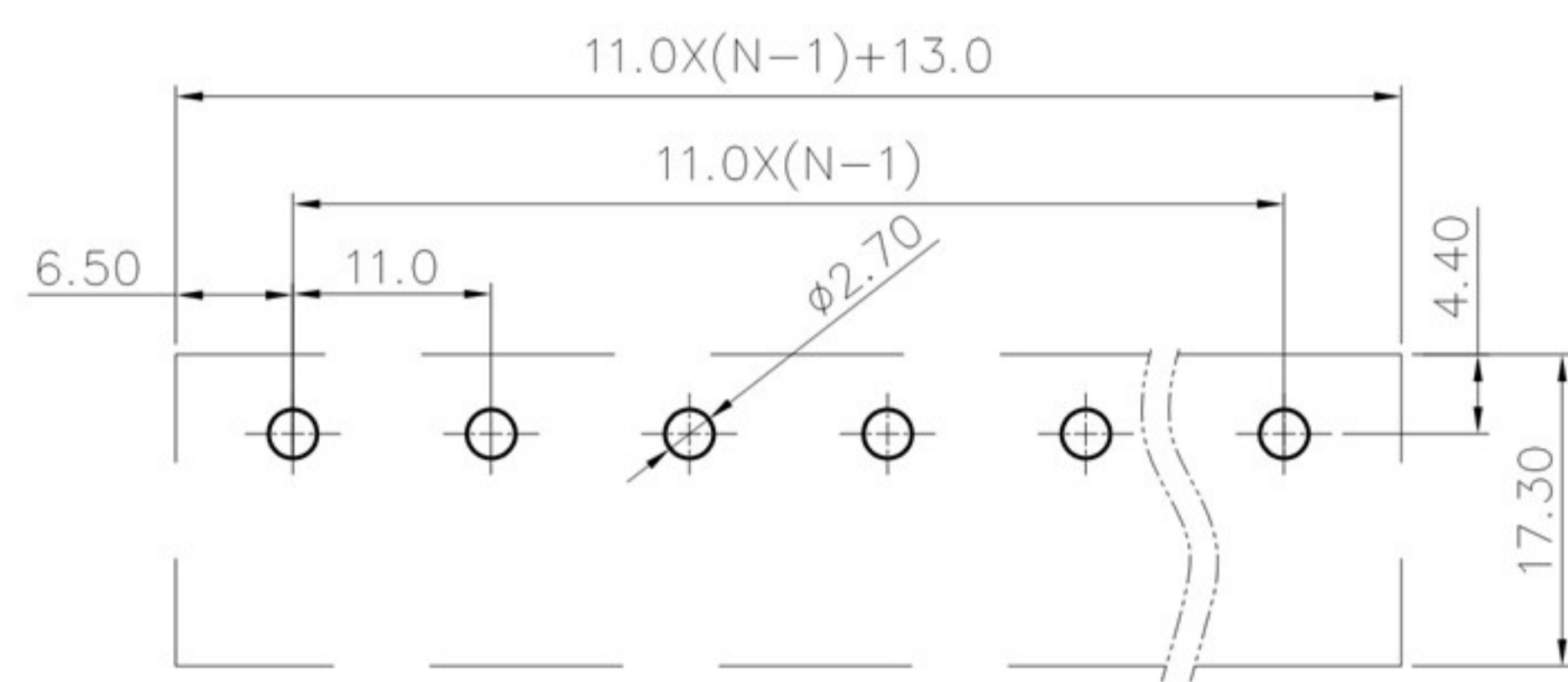
PCB LAYOUT
