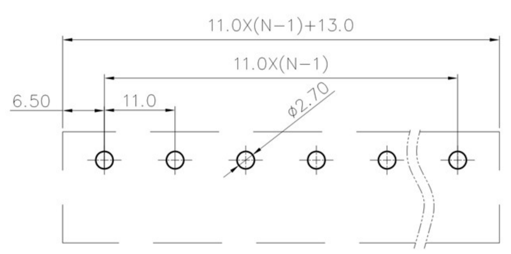
PCB LAYOUT
