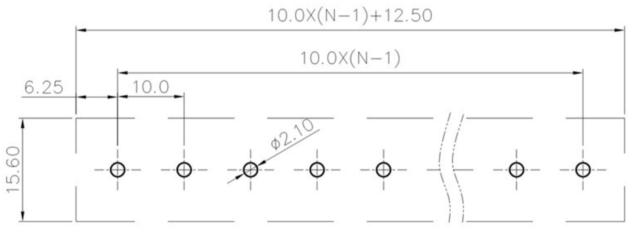
PCB LAYOUT
